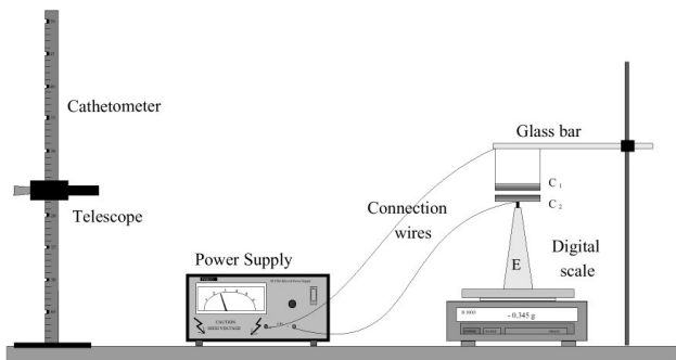
FIGURE 1. Experimental arrangement for the measurement of forces between two parallel conducting cylinders.
