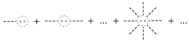
FIGURE 2. Feynman diagrams for the static ghosts contribution to the nonpolynomial term. Dashed and dotted lines represent Higgs bosons and ghosts, respectively.
