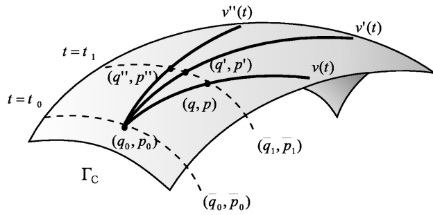
FIGURE 1. Time evolution of a gauge system. \Gamma_C is the constraint surface defined by all first-class constraints. Continue and dashed lines represent histories and orbits, respectively.
