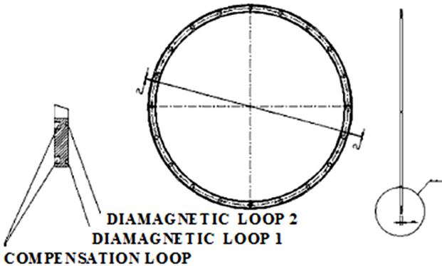
FIGURE 2. The structure of the magnetic arrays.
