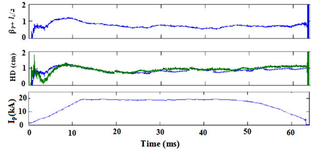
FIGURE 3. The calculated time evolution of the plasma displacement and \beta_p + l_i/2 for circular cross section HT-7 tokamak (green measured by discrete coils and blue calculated).
