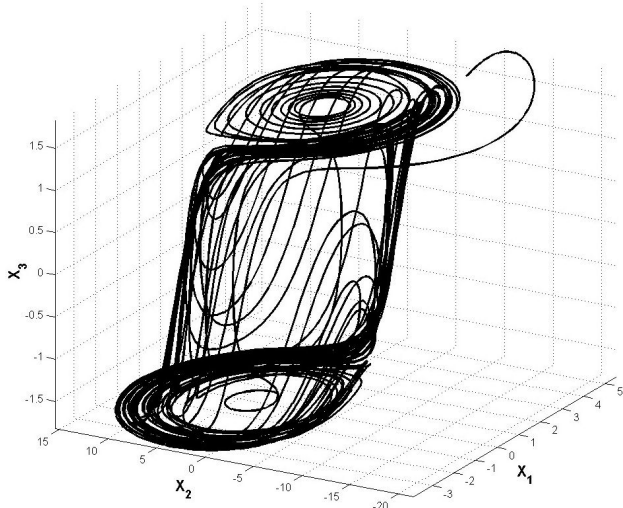
FIGURE 1. Chaotic attractor of the Hysteretic circuit chaotic oscillator projected onto the (x_1, x_2, x_3) -space.
