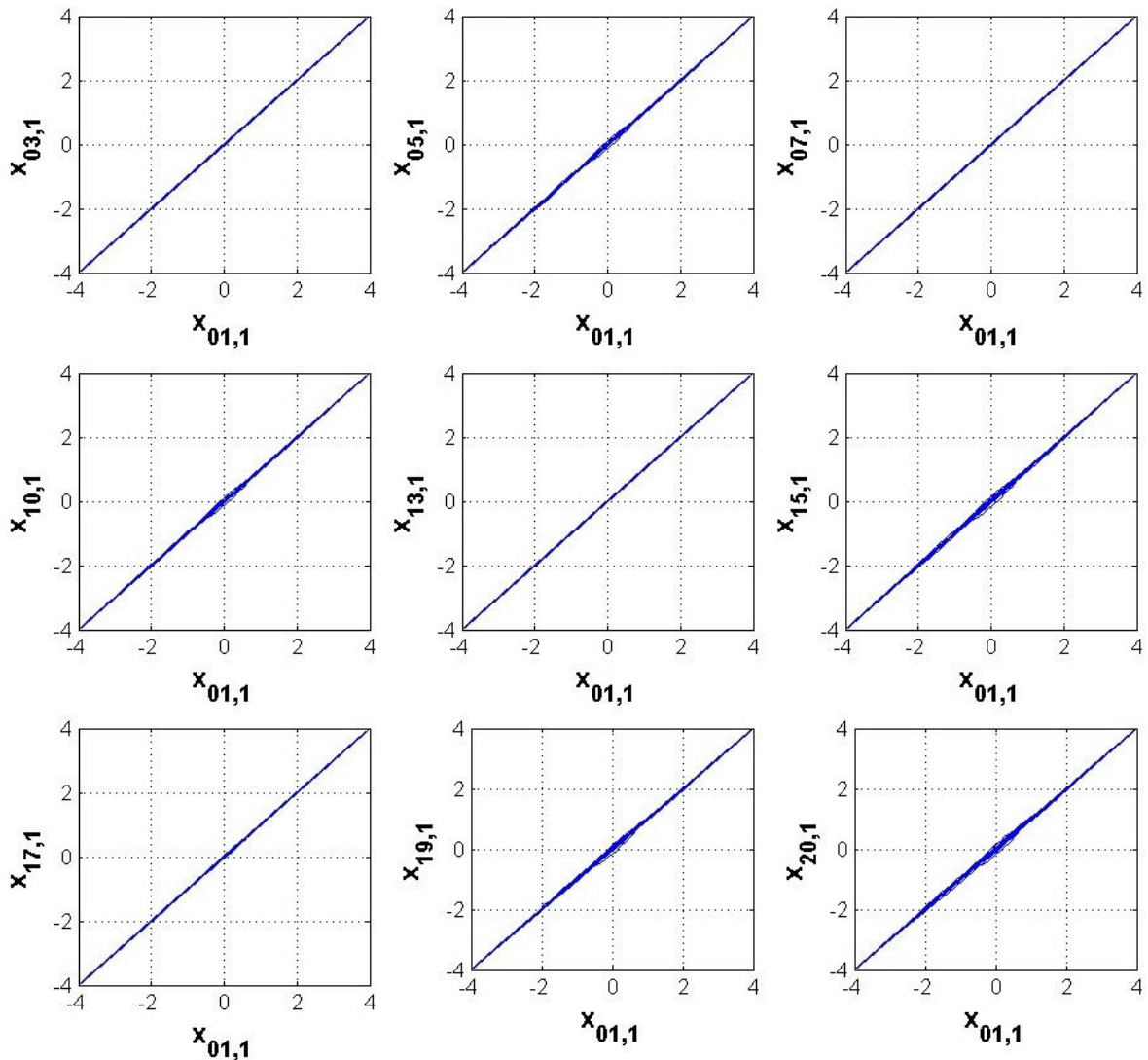
FIGURE 3. Phase plane of the state x_1 of the oscillators 3, 5, 7, 10, 13, 15, 17, 19, and 20 compared to state x_1 of oscillator 1. The phase plane depicts synchronization among the oscillators. Note that only a fraction of the oscillators were compared. These were picked arbitrary and for space purposes. Also note that the synchronization transitory was omitted.
