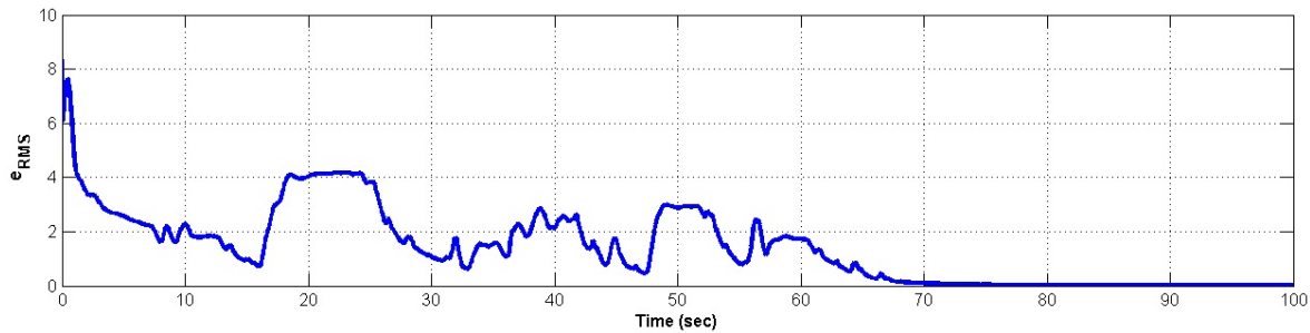
FIGURE 4. Root mean squared error e_{RMS} of the dynamics of every oscillator on the network. Note that only the first 100 seconds are shown.
