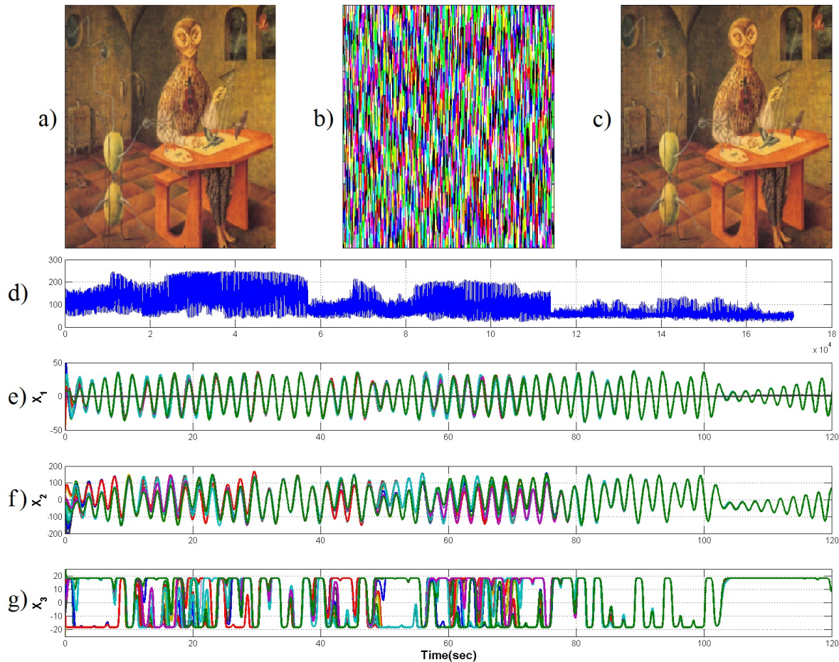
FIGURE 8. a) Depicts the original painting to be encrypted; b) reconstructed image after encryption s(t) = x_{1,2}(t) + m(t) ; c) image reconstructed from oscillator 2 by m^*(t) = s(t) - x_{2,2}(t) . Note that the reconstructed image from oscillator 3 to 20 are the same as in oscillator 2, so then they are not shown. d) Signal produced by reshaping the image, m(t) ; e), f), and g) show the evolution and synchronization of the states x_{i,1}(t) , x_{i,2}(t) , and x_{i,3}(t) respectively, of the oscillators 1 through 20. Note that only the first 120 seconds are shown for representative purposes and that in e) the black line represents the message to be encrypted m(t) as it starts after the synchronization is completed.
