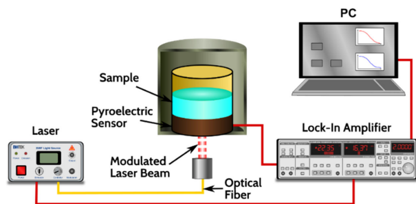
FIGURE 2. Photopyroelectric setup.
