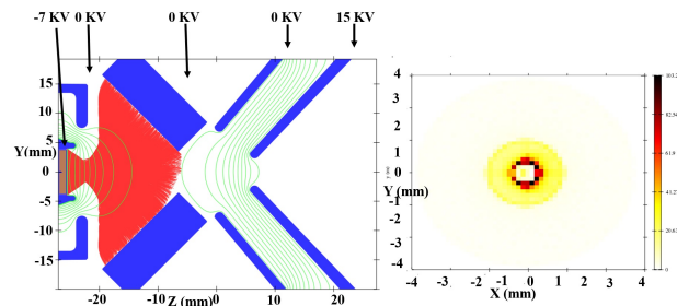
FIGURE 7. IBSIMU simulation: Conical Ionizer producing Cs beam (red) to irradiate the cathode (left) and the irradiation profile at the cathode surface (right).
