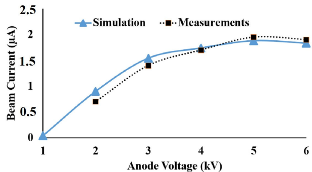
FIGURE 8. H - beam intensity recorded at the Faraday cup for measurements and simulations taking in to account the Cs ions to produce the beam.
