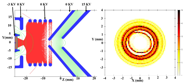
FIGURE 6. IBSIMU simulation: Suppression of the Cs + emission at the Solenoid ionizer surface due to space charge screening (left), and the irradiation profile at the cathode surface (right).
