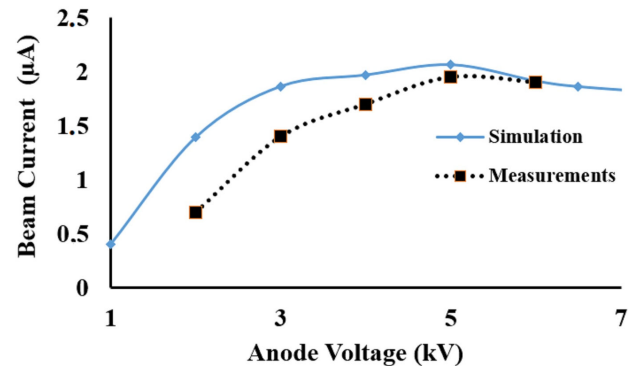
FIGURE 3. H - beam intensity recorded at the Faraday cup vs anode voltage.
