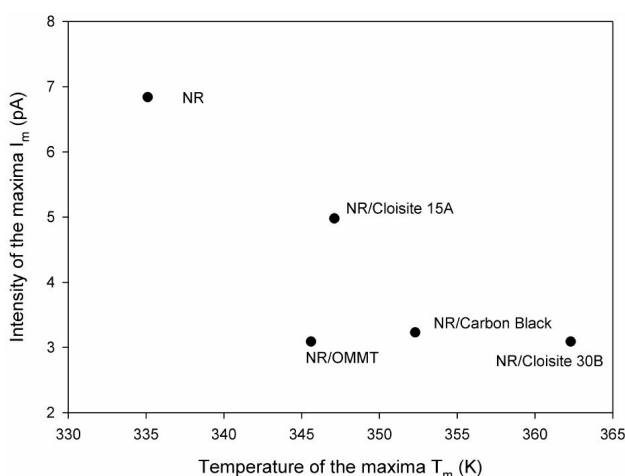
FIGURE 9. Plot of current maxima against peak temperature.
